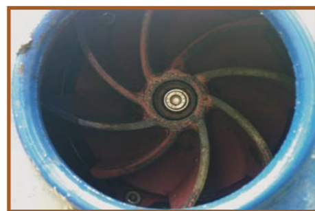
Rag-free pump impeller after 2 months of DERAGGER II ® anti-ragging device operation.
